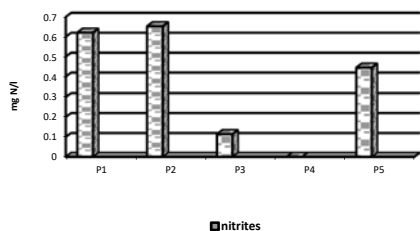
Fig. 5 Nitrites variation in experimental units - using zeolite as filter
