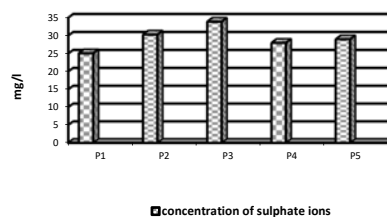
Fig. 12 Sulphate ions variation in experimental units - using zeolite as filter
