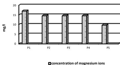
Fig. 9 Magnesium ions variation in experimental units - using zeolite as filter
