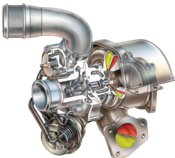
Fig. 2. Turbocharger with twin entry turbine
