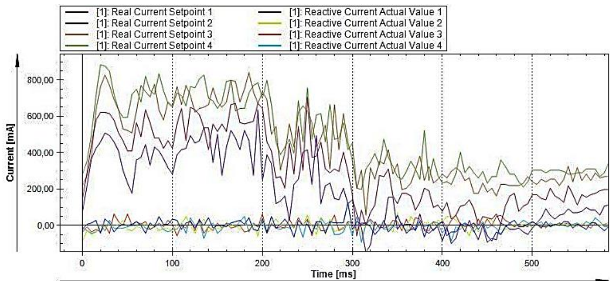
Fig. 2 Energy consumption in the mechatronic module of linear displacement during the operation of pushing a row according to the optimal law of motion (mass of 4 packages 2 kg, distance 270 mm) with the angle of inclination of the plane:: 1- 0^{\circ} ; 2- 30^{\circ} ; 3- 60^{\circ} ; 4- 90^{\circ} .
