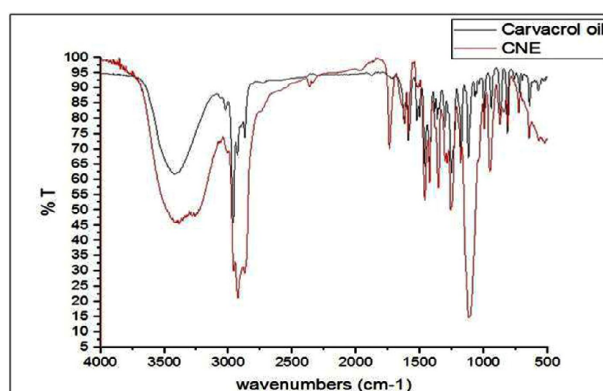
Fig. 3. Fourier-transform infrared spectroscopy (FTIR) of carvacrol essential oil and its nano-emulsion.
