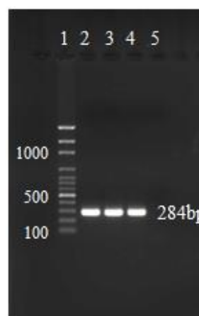
Figure 1. Agarose gel electrophoresis image of PCR products.
