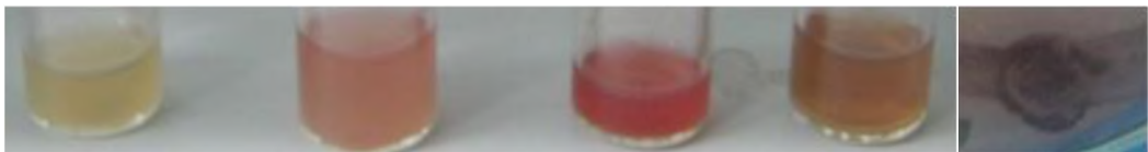
Figure 3: Results of some stages of the biochemical identification of the isolated strain (a – for nitrate reductase; b – for indole; c – with methyl red; d – reaction of Voges-Proskauer; e – for oxidase).
