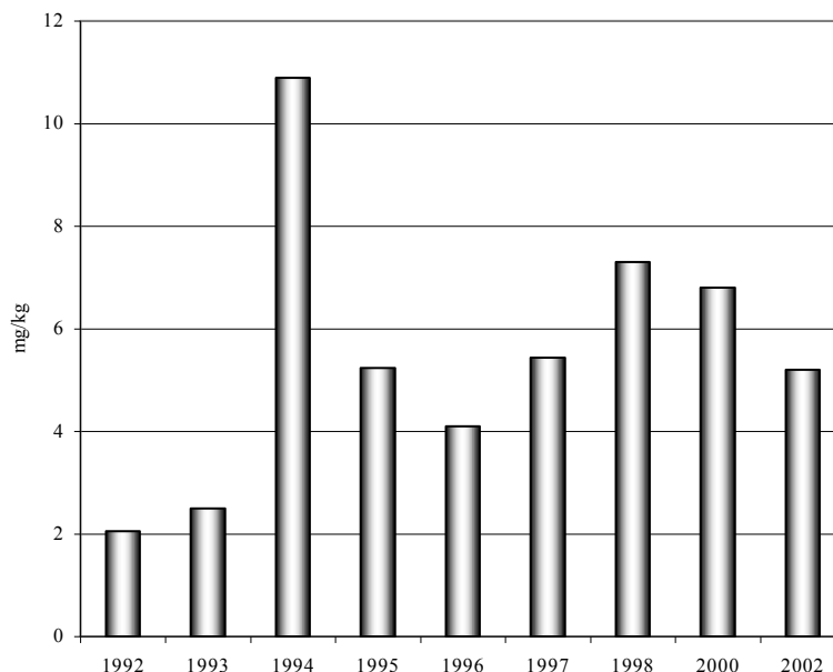
Fig. 2. Long-term monitoring of paradichlorobenzene in Swiss commercial beeswax.
