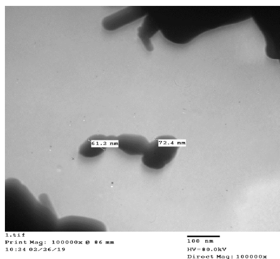
Fig. 2. TEM graph of the synthesised ZnO NPs.
