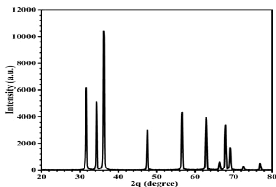
Fig. 1. XRD pattern of the synthesised ZnO NPs.
