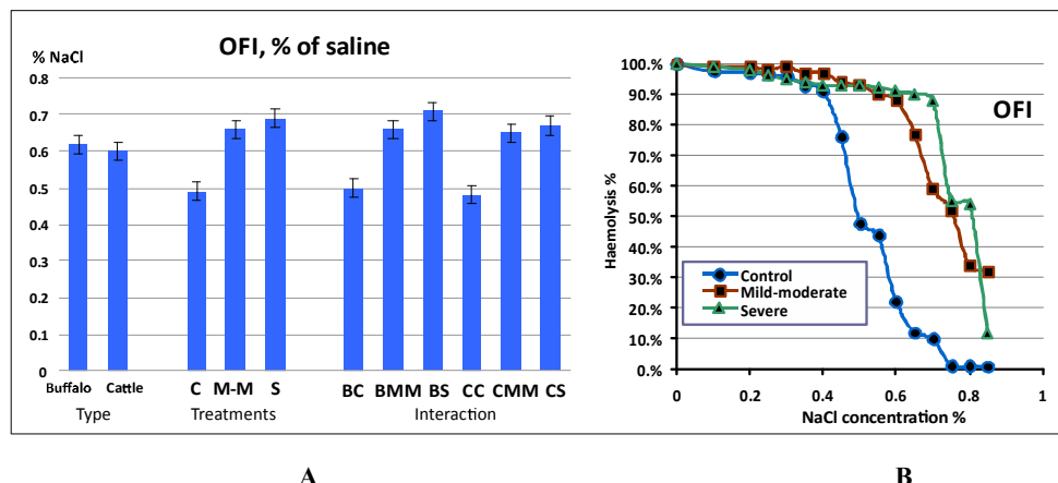
Fig. 3. A. Osmotic fragility Index (mean \pm SD % of saline) in healthy and diseased animals; B. Plots demonstrating osmotic fragility index (OFI) in healthy and diseased animals. C (control), M-M (mild-moderate), S (severe), BC (buffalo control) BMM (buffalo mild-moderate), BS (buffalo severe), CC (cow control), CMM (cow mild-moderate), CS (cow severe).
